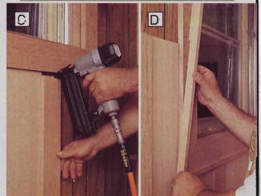
Align the mullions, as in Photo A , to check your layout. The inset shows how to hold them before you're ready to nail. Slide the panels into place, as in Photo B . Fit the window trim pieces, as in Photos C and D .
